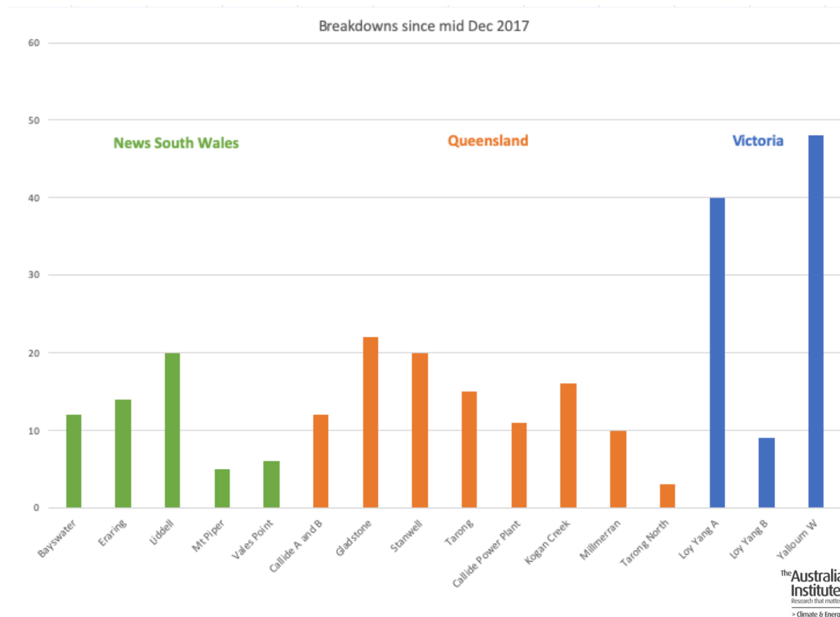
Figure 2: Coal power station outages in the NEM, December 2017 – 2020
